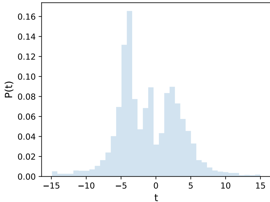
hist(t, bins="freedman")
