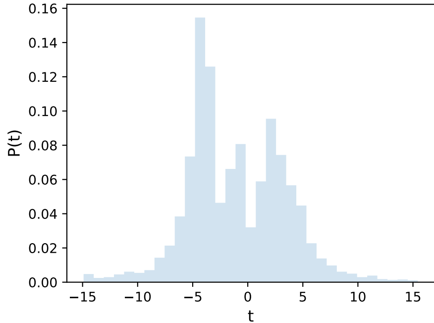
hist(t, bins="scott")
