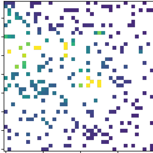
Sparsely Sampled
