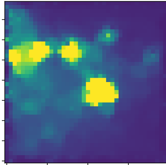
Reconstructed
