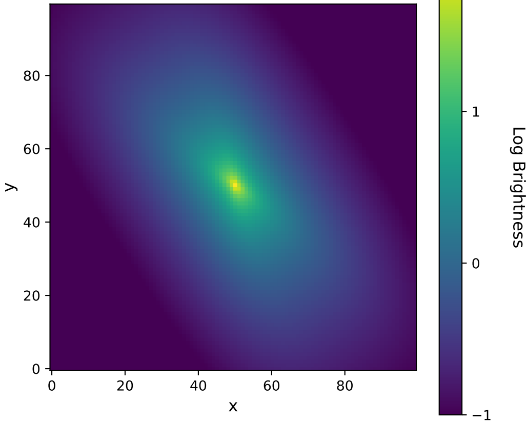
Boxy isophote with c=1.0
