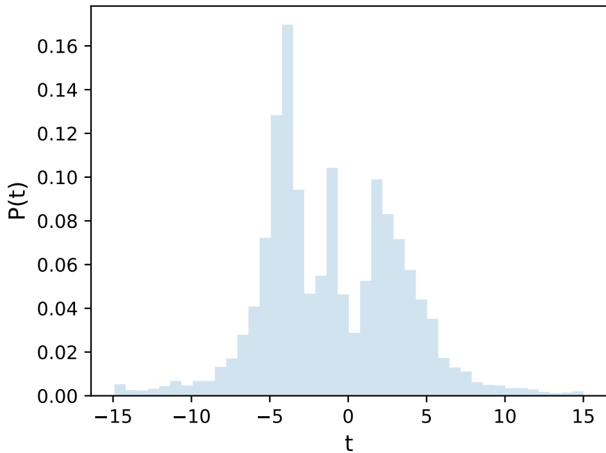
hist(t, bins="knuth")
