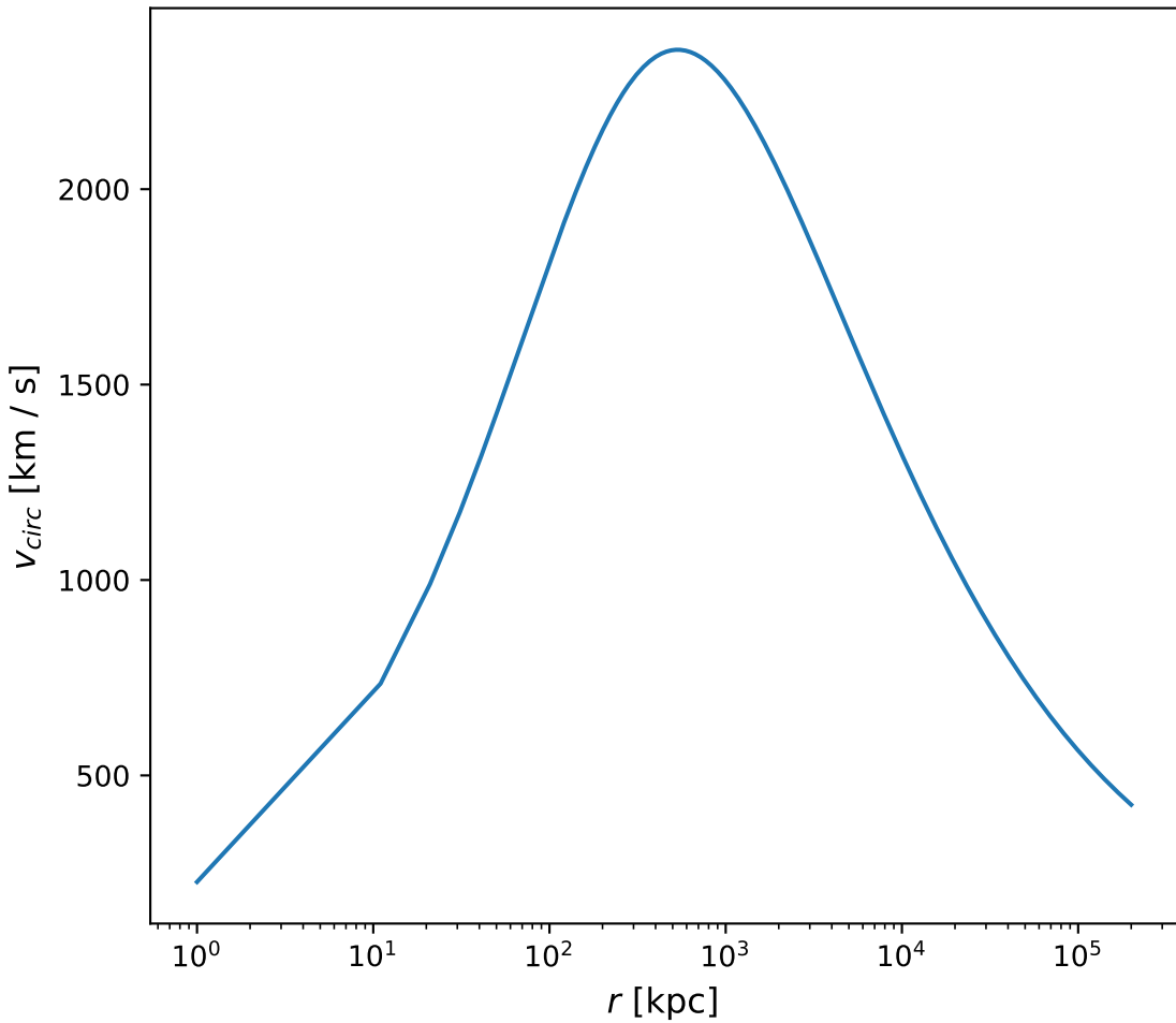
NFW Profile Circular Velocity
