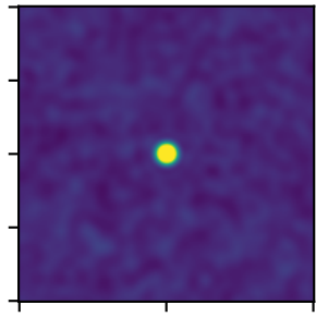
AiryDisk2DKernel
