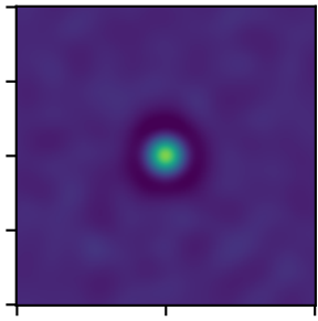
RickerWavelet2DKernel
