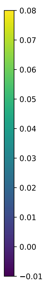
Gaussian2DKernel
