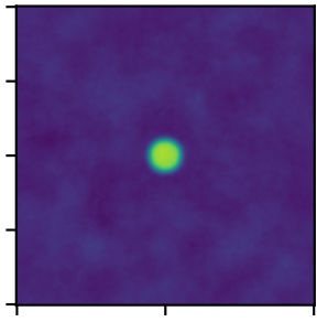
Tophat2DKernel
