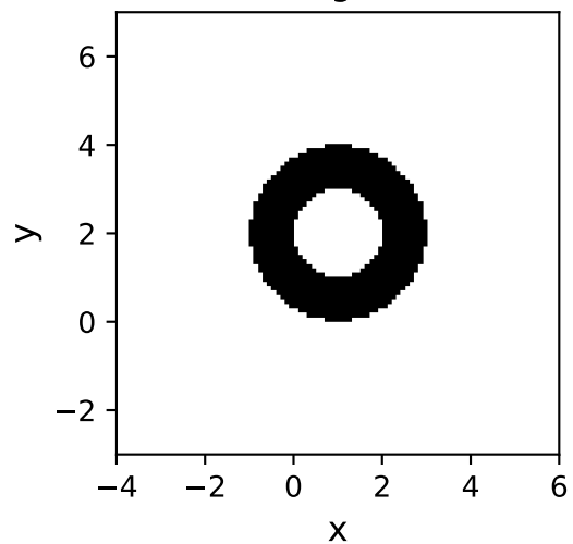
Ring2D
