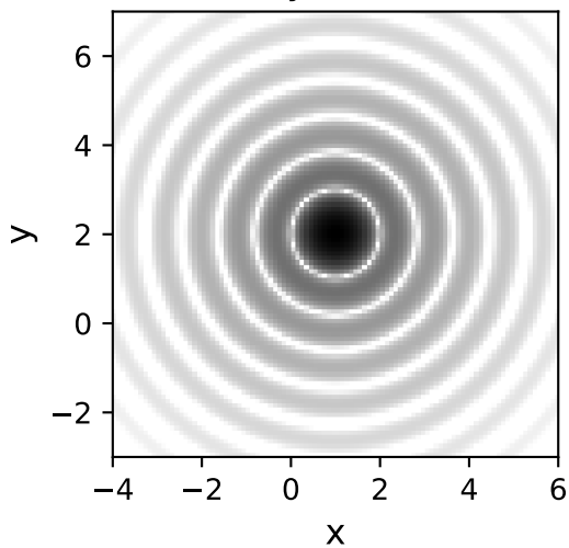
AiryDisk2D
