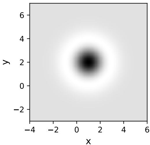
RickerWavelet2D
