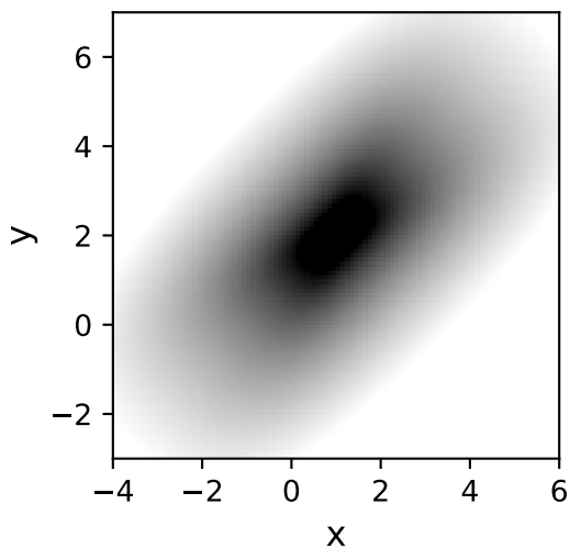
GeneralSersic2D, c=1.0
