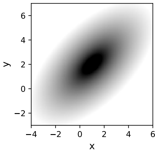
Sersic2D
