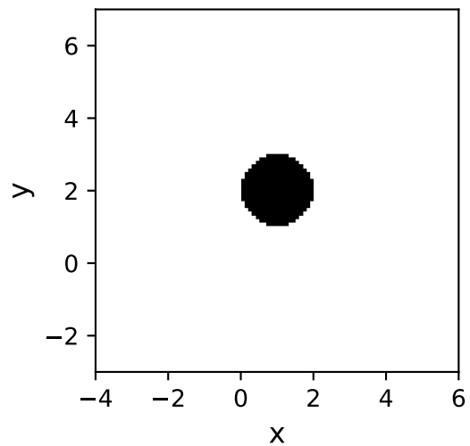
Disk2D
