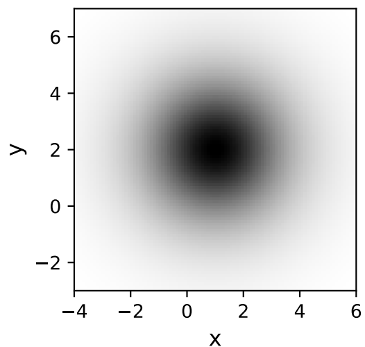
Moffat2D
