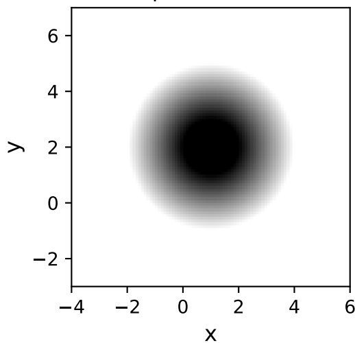
TrapezoidDisk2D
