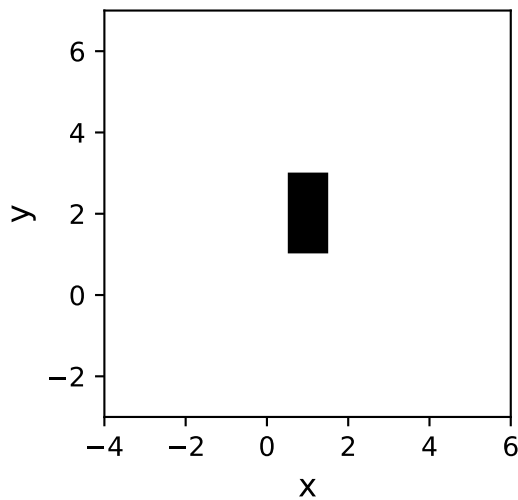
Box2D
